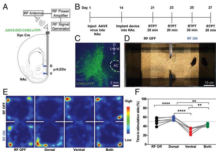
Fig. 6. Multichannel optogenetic activation of reward and aversion. ( A ) Cartoon of directionally controlled light spread of \mu -ILED devices for isolating subregions of NAcSh. ( B ) Experimental paradigm for testing optogenetic control of reward and aversion. ( C ) Confocal micrograph of virally induced ChR2 expression in dynorphin-expressing neurons in the NAcSh. Nissl cell body stain is blue, and ChR2-eYFP native fluorescence is green. ( D ) Photo of the real-time place testing assay. ( E ) Representative heat map of time spent in the stimulation (rf-on) side following no stimulation, dorsal or ventral wireless photostimulation, and dorsal and ventral photostimulation together. ( F ) Stimulation with dorsal \mu -ILED drives a real-time place preference, but stimulation with ventral \mu -ILED drives an aversion, measured as a significant increase or decrease in time spent in the stimulation side (%), respectively. Stimulating both ventral and dorsal \mu -ILEDs has no significant effect on behavior. Data are represented as mean \pm SEM, n = 6 . One-way ANOVA, Bonferroni post hoc; ****P < 0.0001 rf-off vs. ventral and dorsal vs. ventral; **P < 0.01 dorsal vs. both and ventral vs. both.
